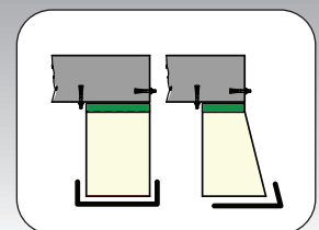
E. Double layer on impact area
