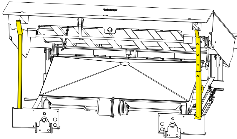
Maintenance Strut
